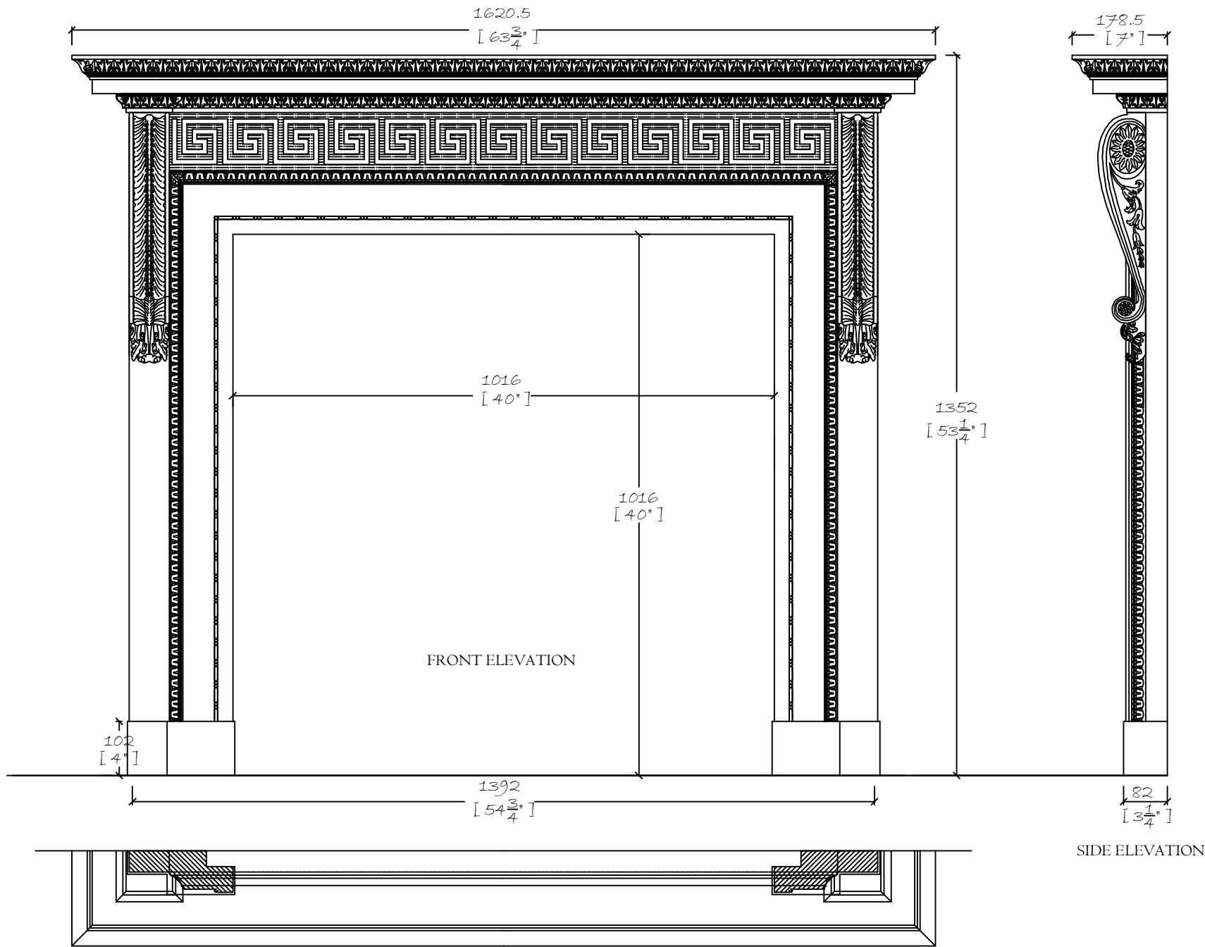
PLAN
