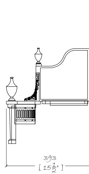
SIDE ELEVATION
