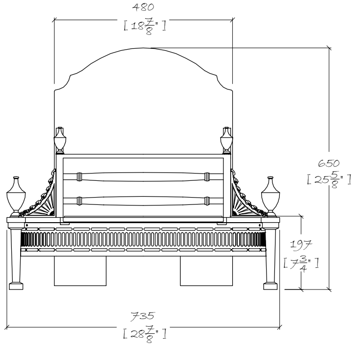
FRONT ELEVATION
