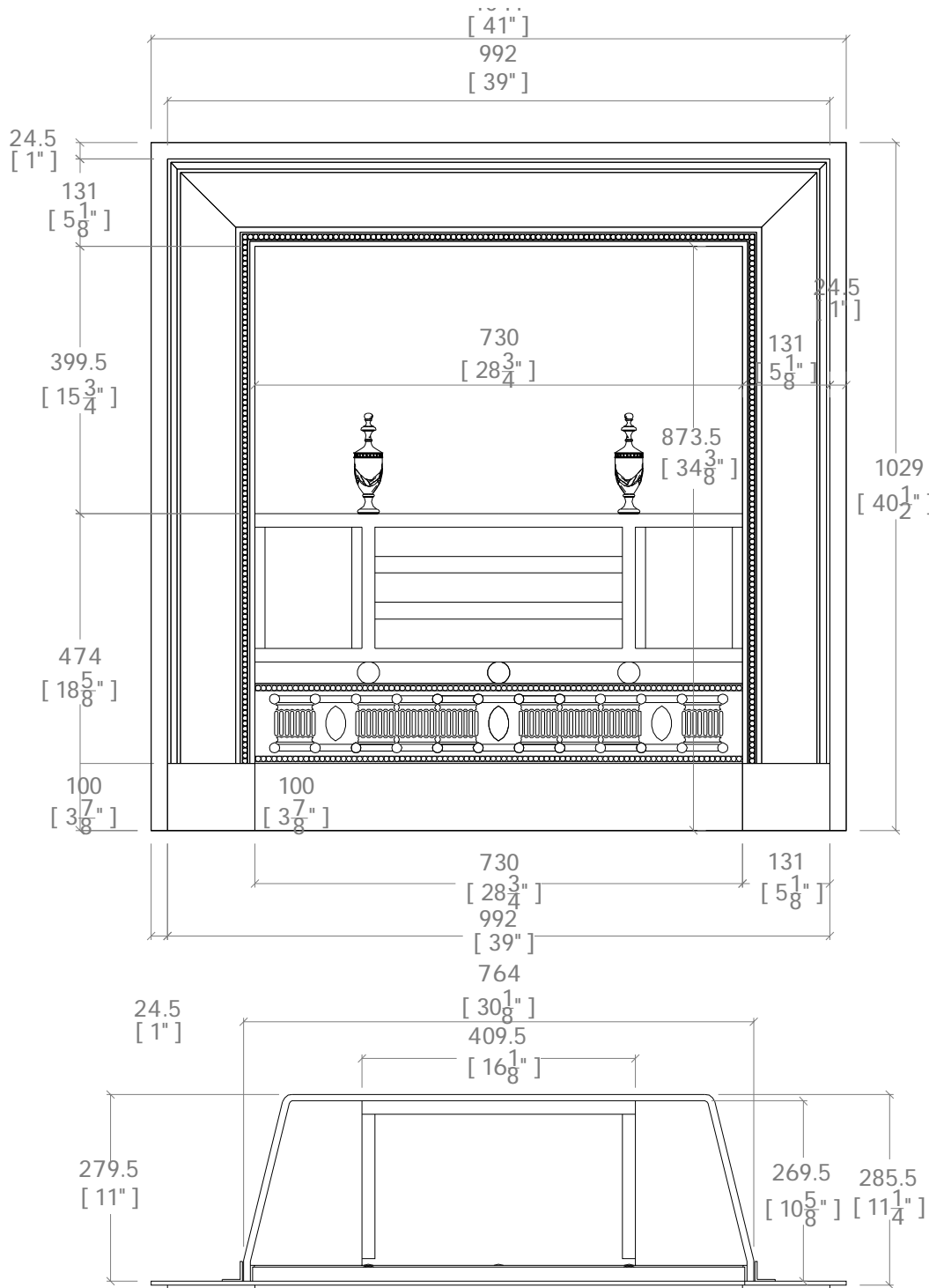
Campbell Date: 05/05/2015 full scale & 1:10 DRAWING NO. 31929D
