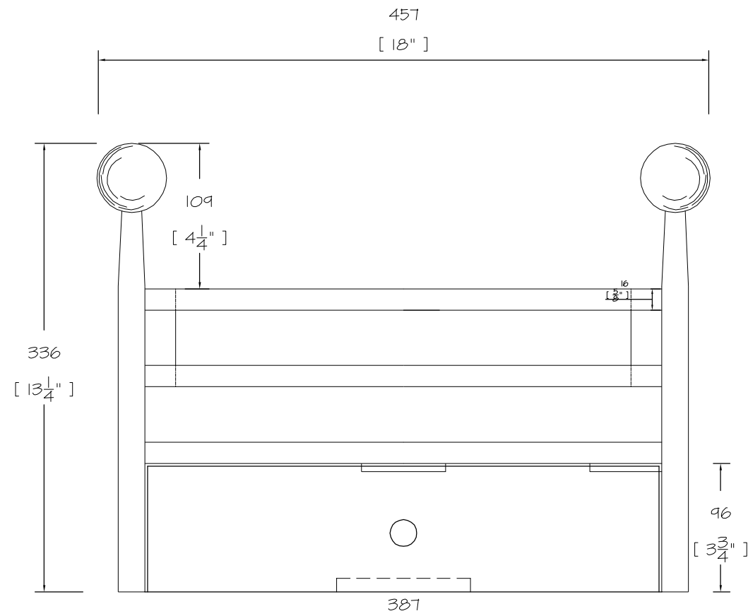
Front Elevation
