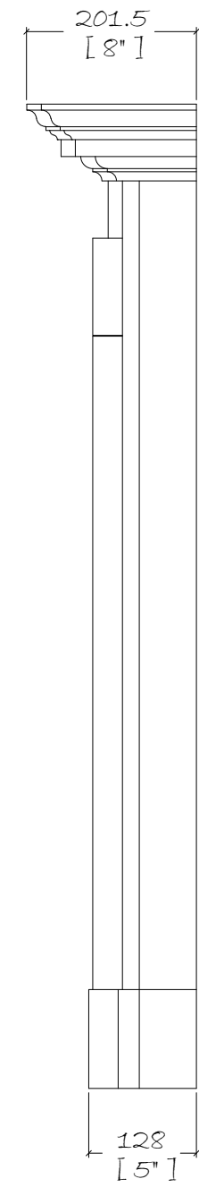
SIDE ELEVATION
