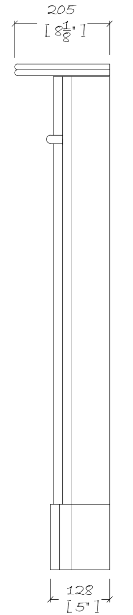
SIDE ELEVATION
