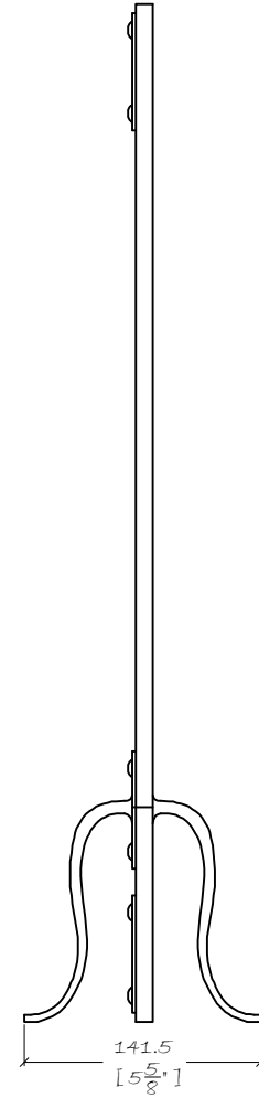
SIDE ELEVATION
