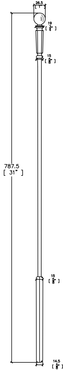
Side Elevation (The Cotswold)
