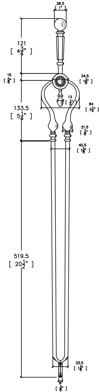
Front Elevation (The Cotswold)
