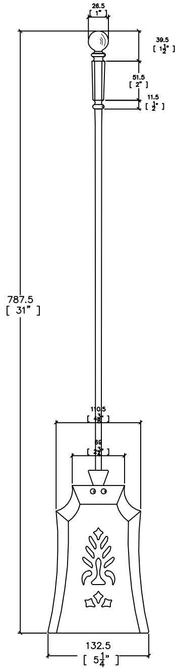
Front Elevation (The Cotswold)
