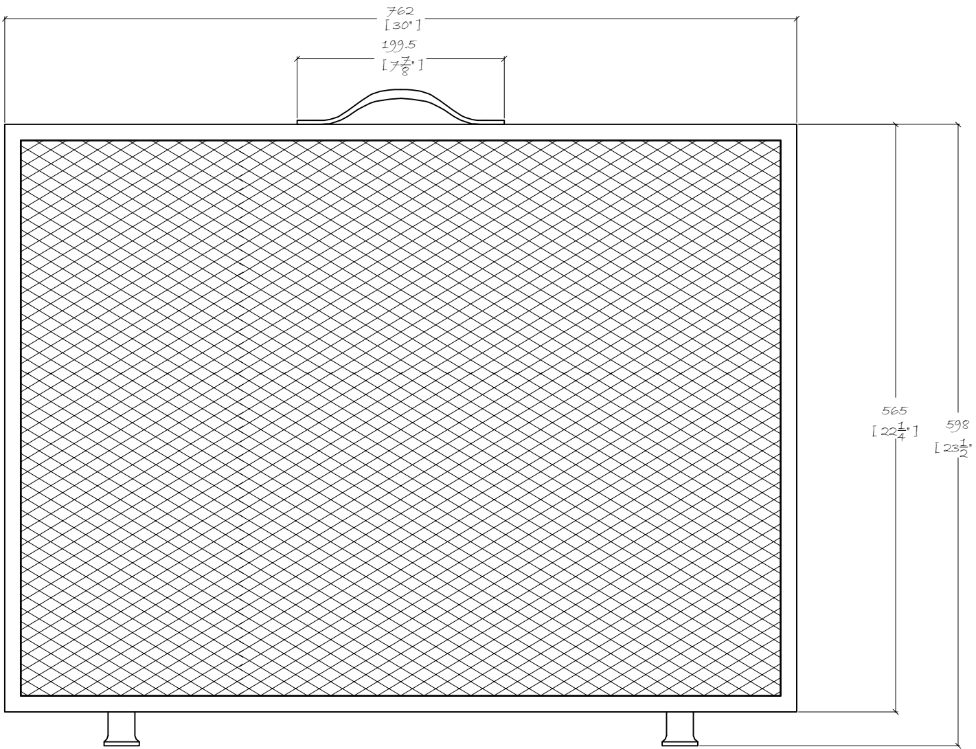
FRONT ELEVATION
