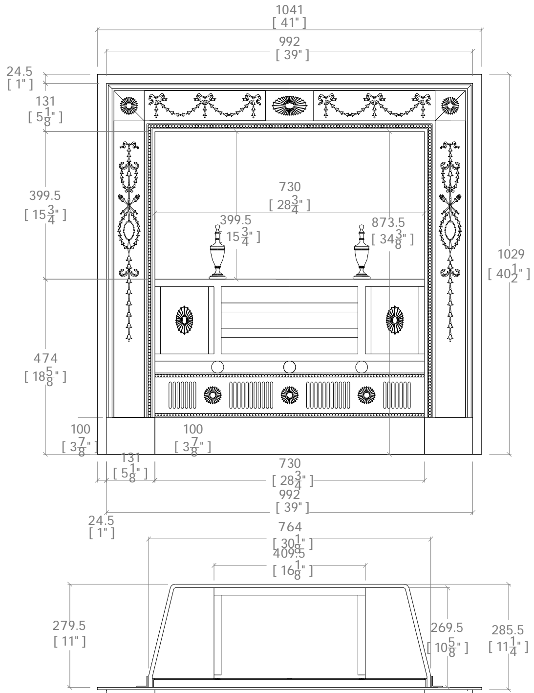
Hawksmoor Date: 05/05/2015 full scale & 1:10 DRAWING NO. 31932D
