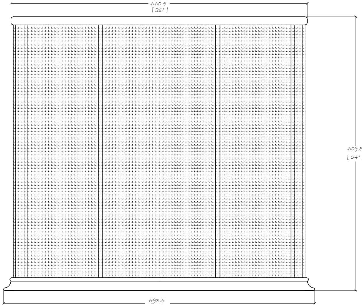
FRONT ELEVATION
