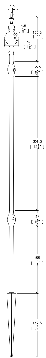
Front Elevation (The Ridings)
