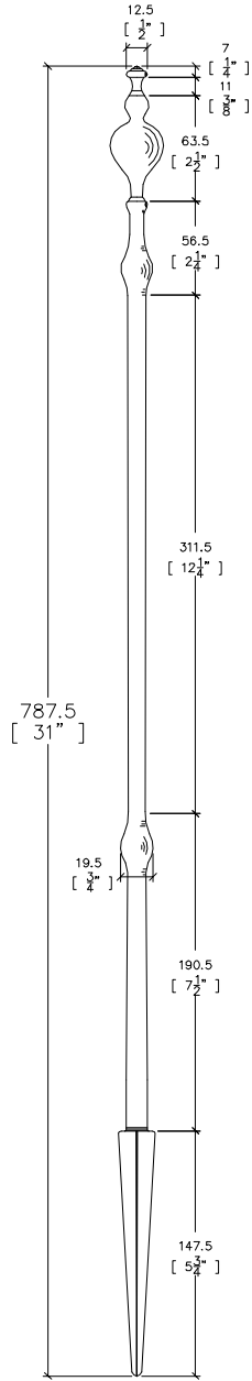
Side Elevation (The Ridings)
