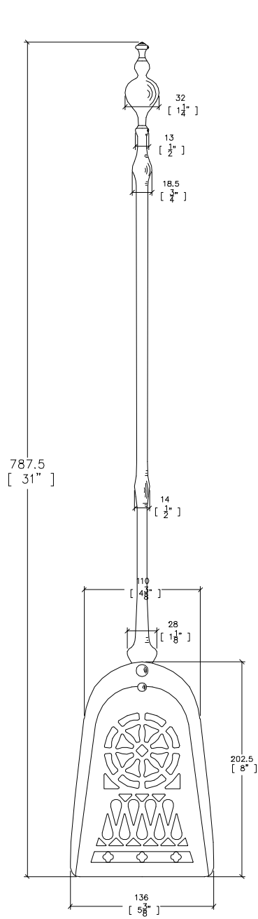
Front Elevation (The Ridings)
