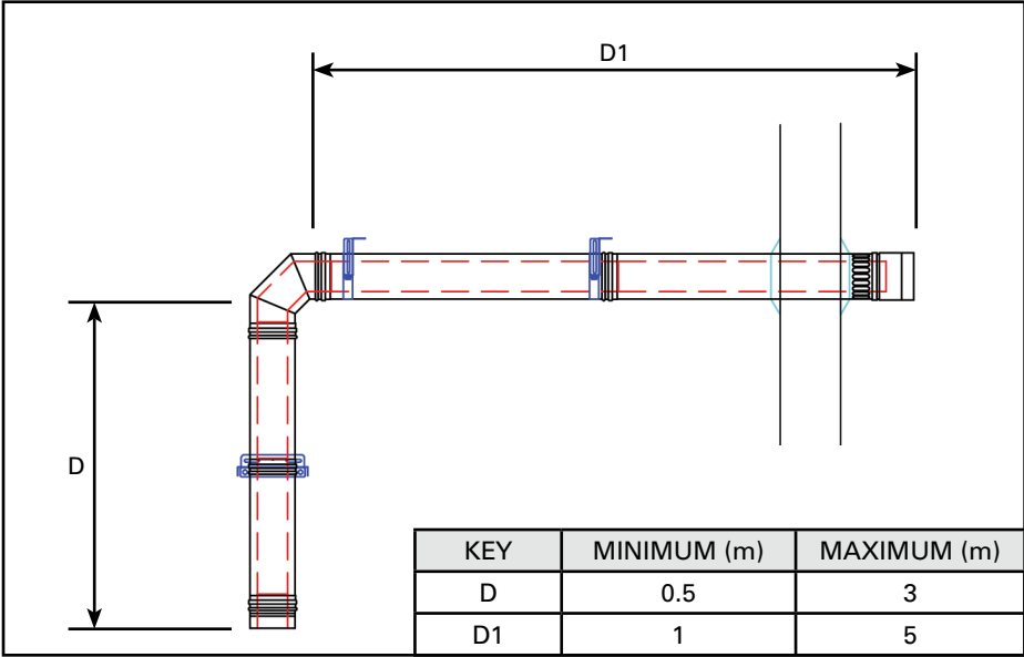
Horizontal Wall Vent Termination Fig.18
