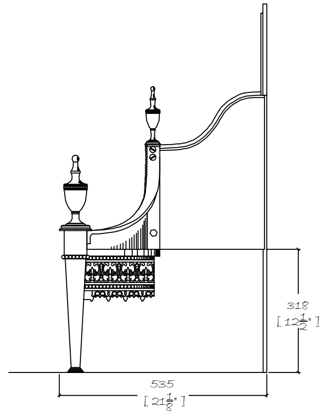
SIDE ELEVATION
