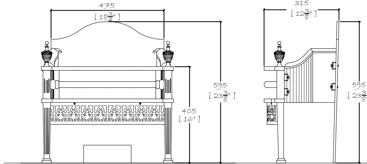
FRONT ELEVATION
