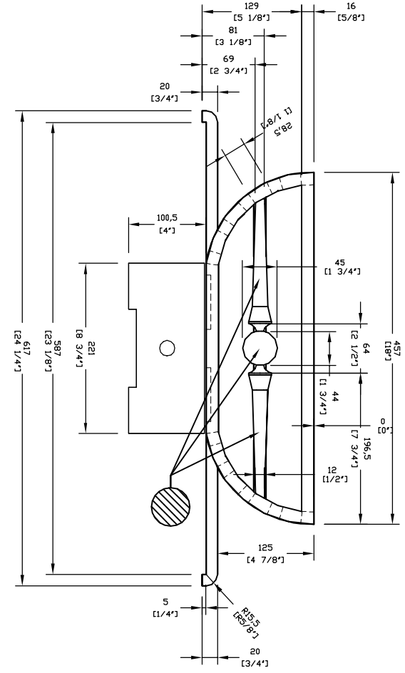
Front Elevation
